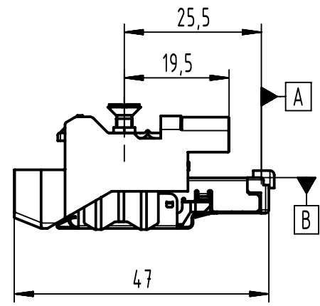
Han 3A adaptor with closed lever:
